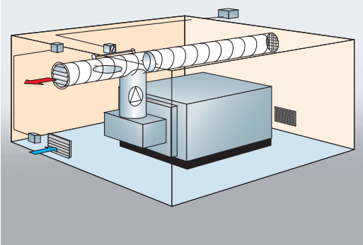
Energy recovery from an air-cooled compressor.
