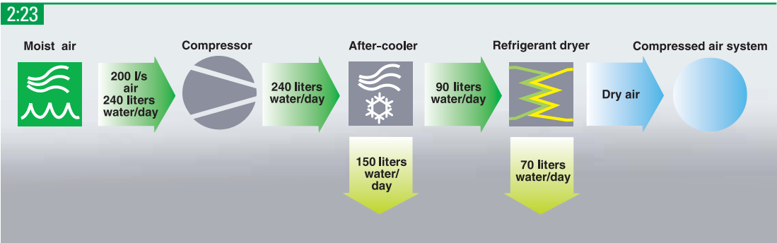
A compressor that delivers 200 liters/second of air also supplies approx. 10 liters/hour of water when compressing air at 20°C. Problems due to water precipitation in the pipes and equipment are avoided by the use of after-cooler and drying equipment.
