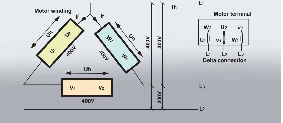
This illustrates the motor windings connected in a delta configuration, and how the connection strips are placed on the delta-connected motor terminal. The example shows the connection to a 400V supply.
