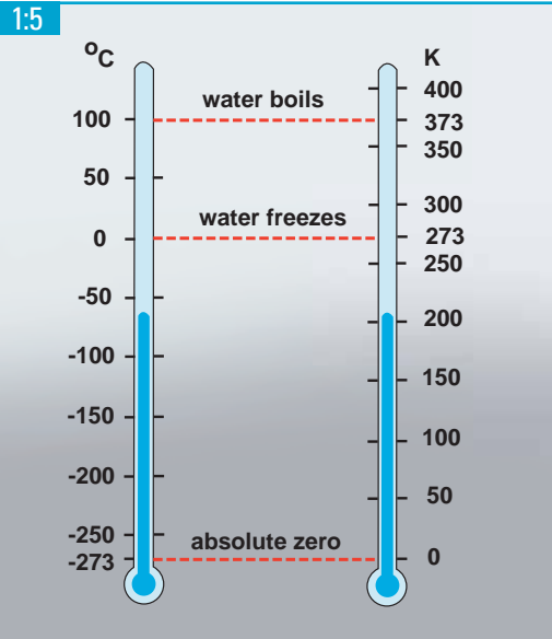
This illustrates the relation between Celsius and Kelvin scales. For the Celsius scale 0° is set at the freezing point of water; for the Kelvin scale 0° is set at absolute zero.
