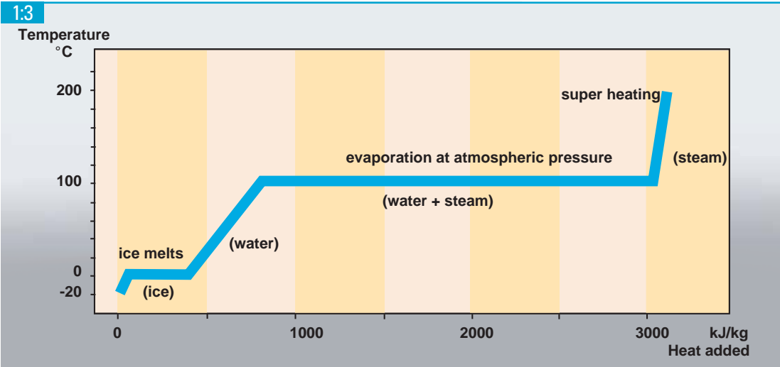
By applying or removing thermal energy the physical state of a substance changes. This curve illustrates the effect for pure water.
