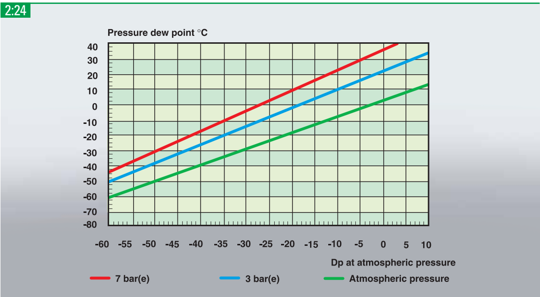
Relation between dew point and pressure dew point.
