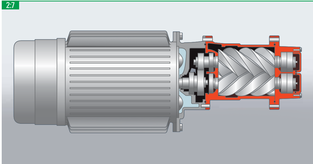
A modern integrated-drive oil-lubricated screw compressor.
