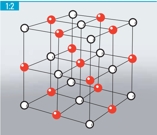
A salt crystal such as common table salt NaCl has a cubic structure. The lines represent the bonding between the sodium (red) and the chlorine (white) atoms.
