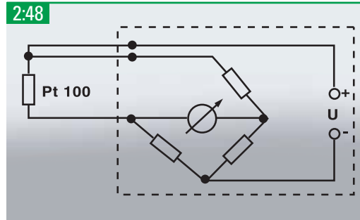
Example of a 3-wire connection using a resistance thermometer of 100Ω. The resistance thermometer and connectors are connected on a bridge.
