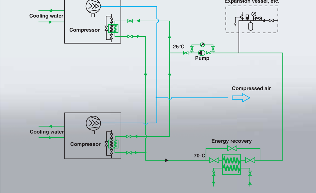
Example of water-borne energy recovery of an oil lubricated screw compressor. The residue cooler with regulation system is integrated in the compressor.
