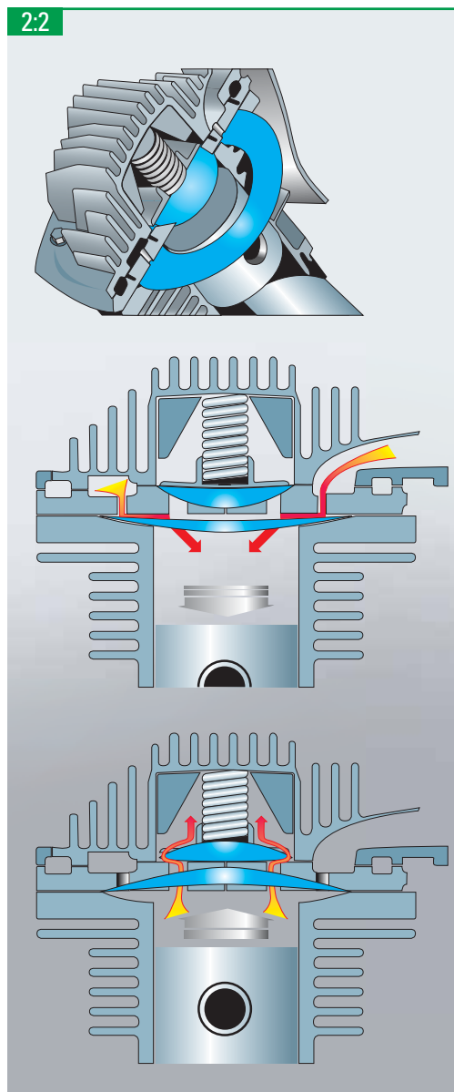
Piston compressor with a valve system consisting of two stainless steel valve discs.
