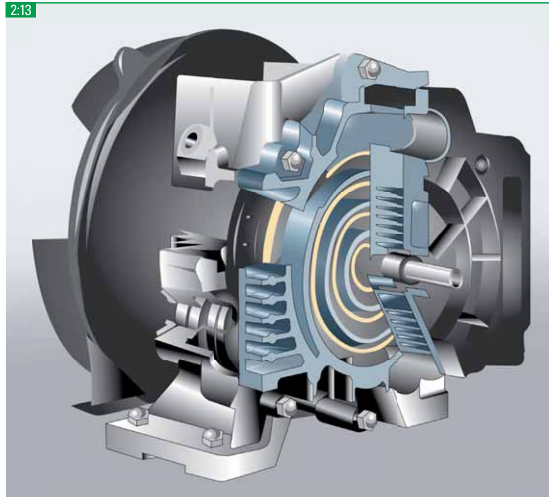
A scroll compressor cross section.
