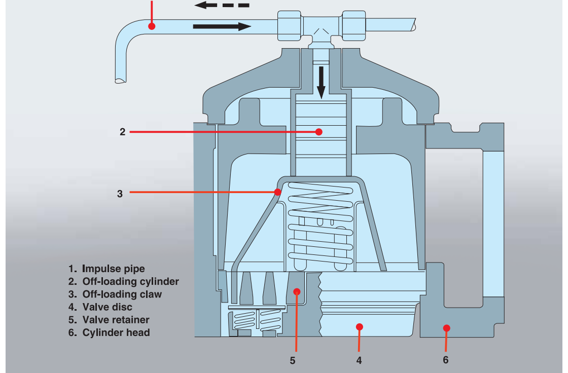
Off-loading device for a piston compressor.
