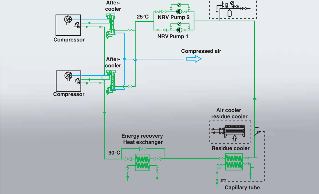
Example of water-borne energy recovery of an oil-free screw compressor.
