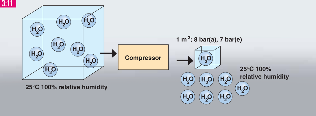
A compressor that works at 7 bar(e) gauge pressure, compresses air to 1/8 of its volume.
