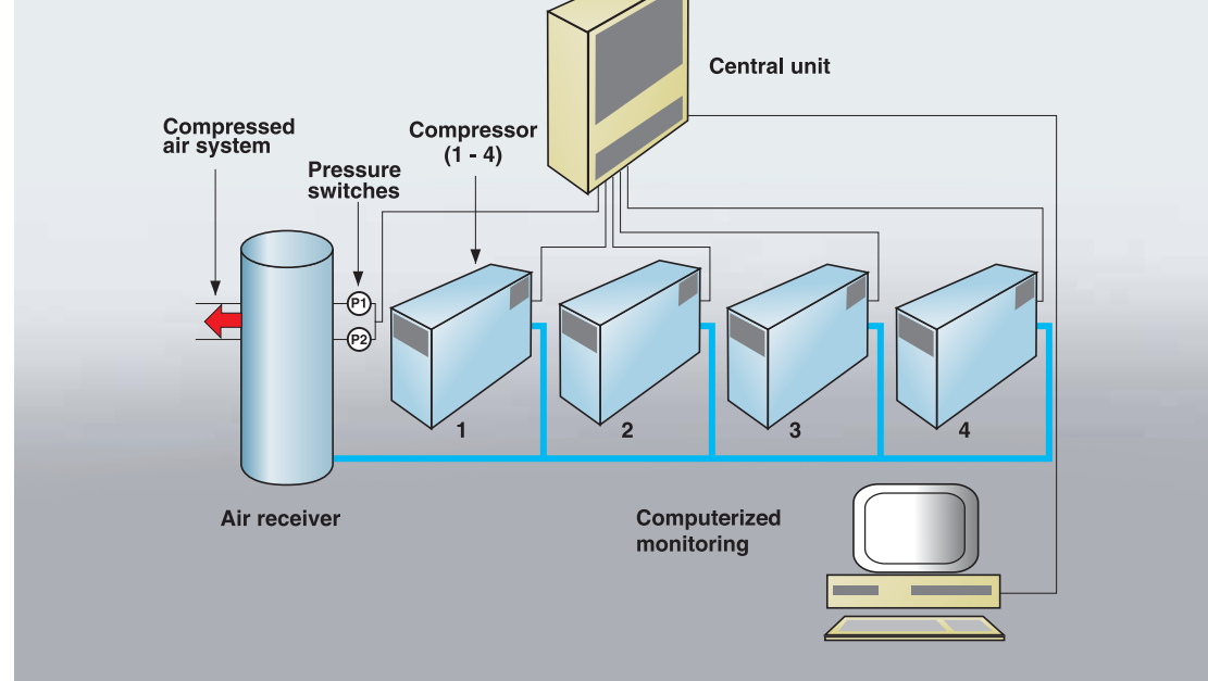
Centrally controlled compressor installation.
