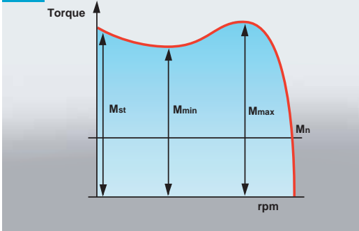
The torque curve for a squirrel cage induction motor. When the motor starts the torque is high. M_{st} = start torque, M_{max} = max torque (“cutting torque”), M_{min} = min. torque (“saddle torque”), M_n = rated torque.
