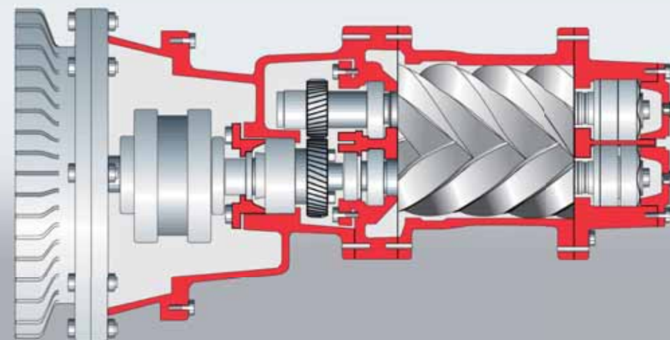
Typical oil lubricated screw compressor element and drive.
