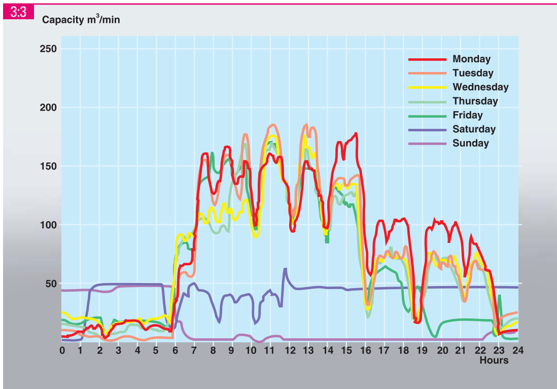
During an operation analysis the compressed air production is continuously measured for a full week.
