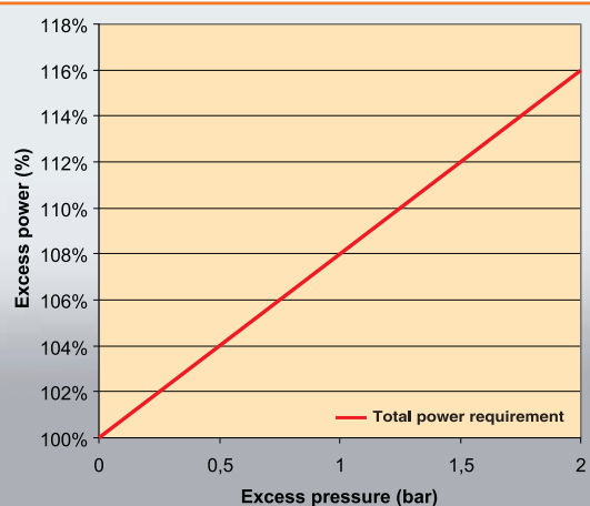
Excess power requirement as a result of over-pressurizing to compensate for pressure drops. For a 300 l/s compressor, raising the working pressure by 1 bar means 6 kW higher power consumption. At 4000 operating hours/year this represents 24,000 kWh/year or € 2,400/year.
