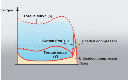
A star/delta started induction motor torque curve combined with a torque demand curve for a screw compressor. The compressor is unloaded (idling) during star operations. When the speed has reached approx. 90-95% of the rated speed the motor is switched to the delta mode, the torque increases, the compressor is loaded and finds its working point.
