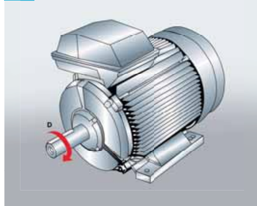
The mains supply is connected to a three-phase motor’s terminals marked U, V and W. The phase sequence is L1, L2 and L3. This means the motor will rotate clockwise seen from “D” the drive end. To make the motor rotate anticlockwise two of the three conductors connected to the starter or to the motor are switched. Check the operation of the cooling fan when rotating anticlockwise.
