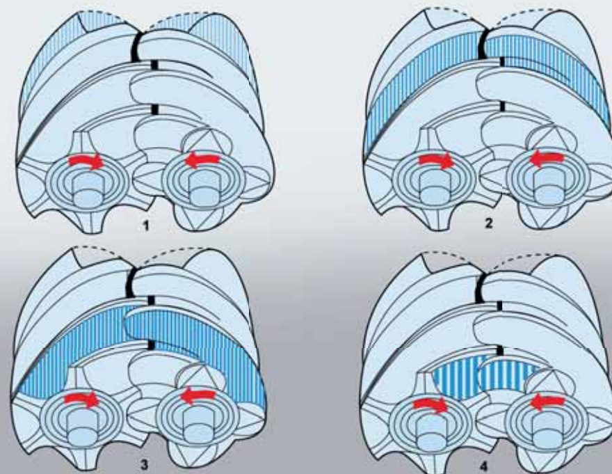
This illustrates compression in a twin screw compressor. Figure 1: air fills the space between the rotors, Fig. 2-4: gradually the enclosed space decreases and pressure increases.
