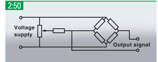
Bridge connection with strain gauges.
