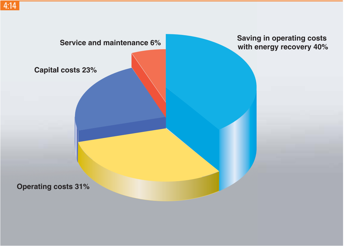
Compressed air cost contributors with energy recovery.
