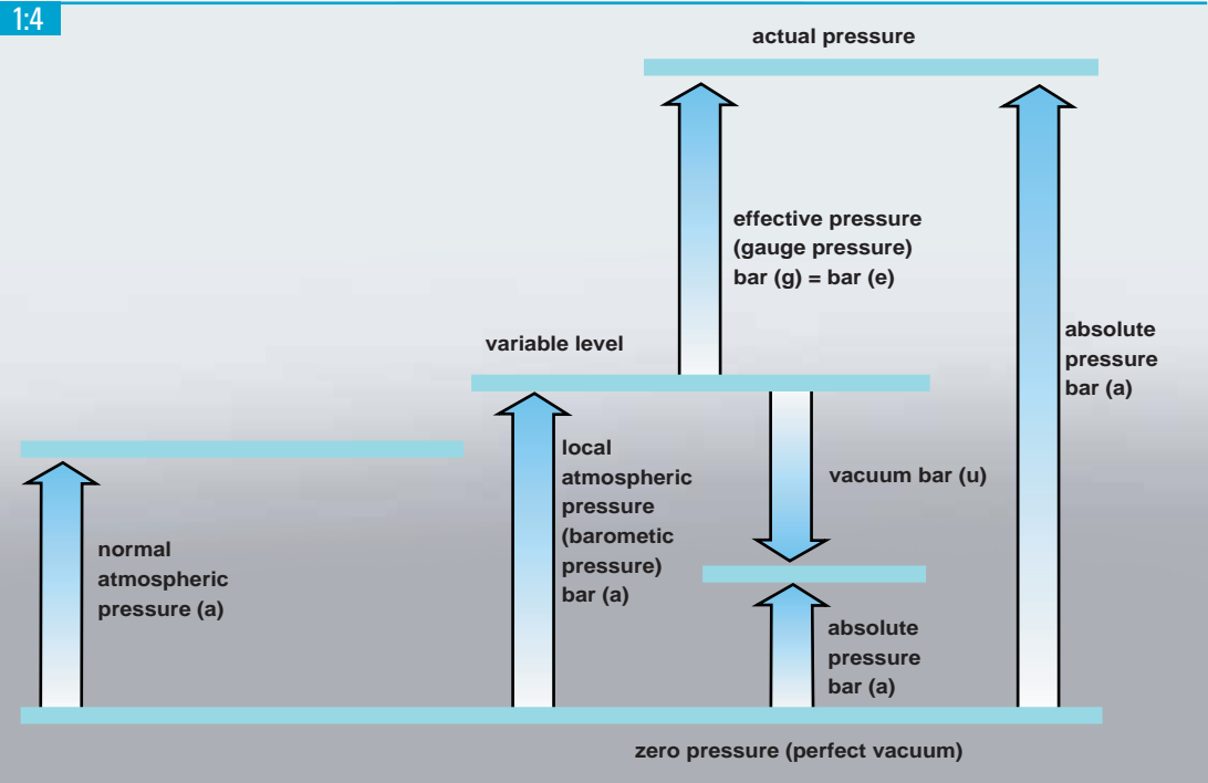
Most pressure gauges register the difference between the pressure in a vessel and the local atmospheric pressure. Therefore to find the absolute pressure the value of the local atmospheric pressure must be added.
