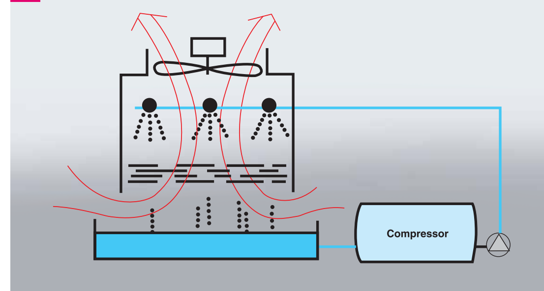
Open cooling system with circulating cooling water.
