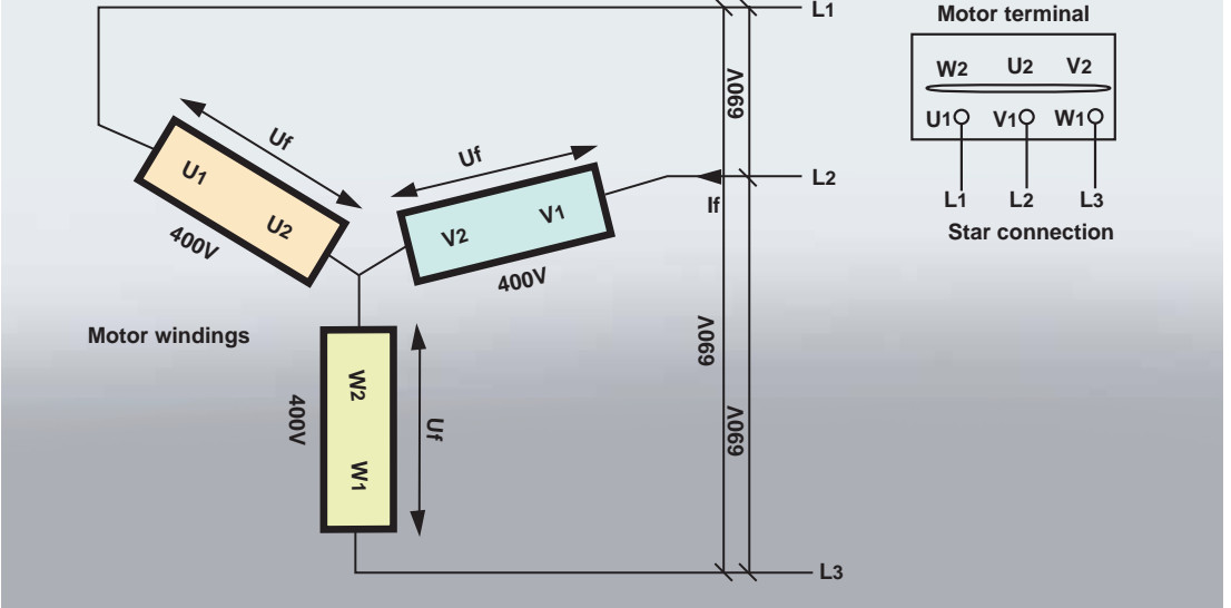
This illustrates the motor windings connected in a star configuration, and how the connection strips are placed on the star-connected motor terminal. The example shows the connection to a 690V supply.
