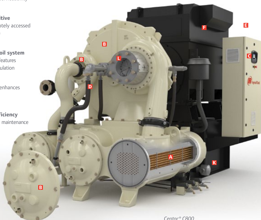
Centac® C800
