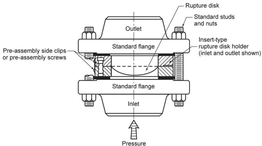
Figure 24—Reverse-acting Scored Rupture Disk
