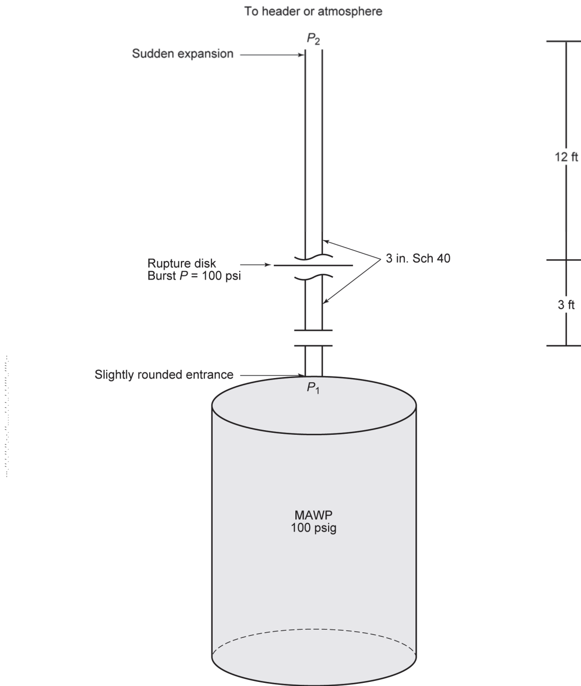
Figure E.1—Pressure-relief System for Example Problem
