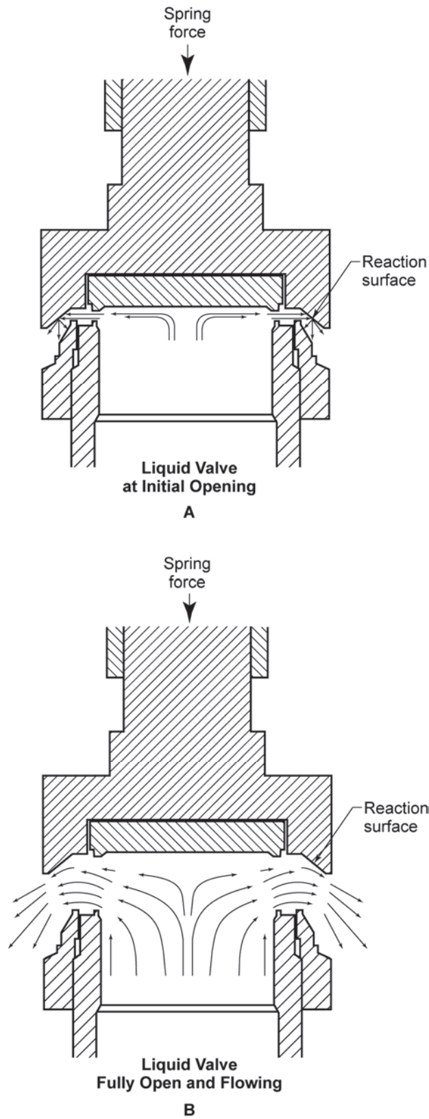
Figure 7—PRV Operation—Liquid Service
