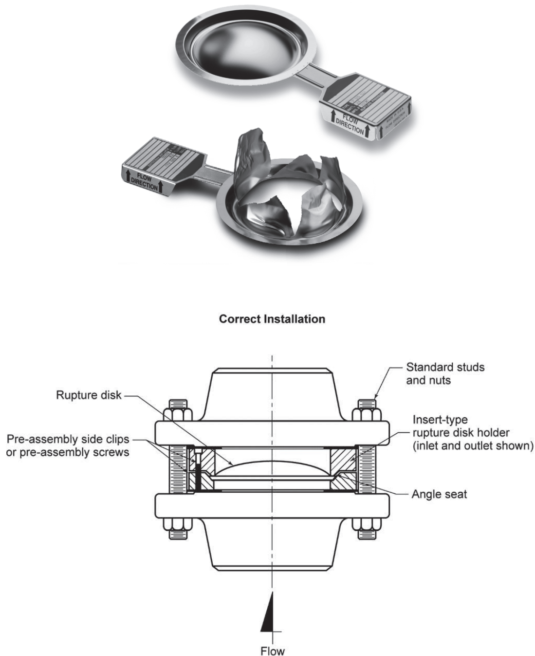
Figure 20—Forward-acting Solid Metal Rupture Disk
